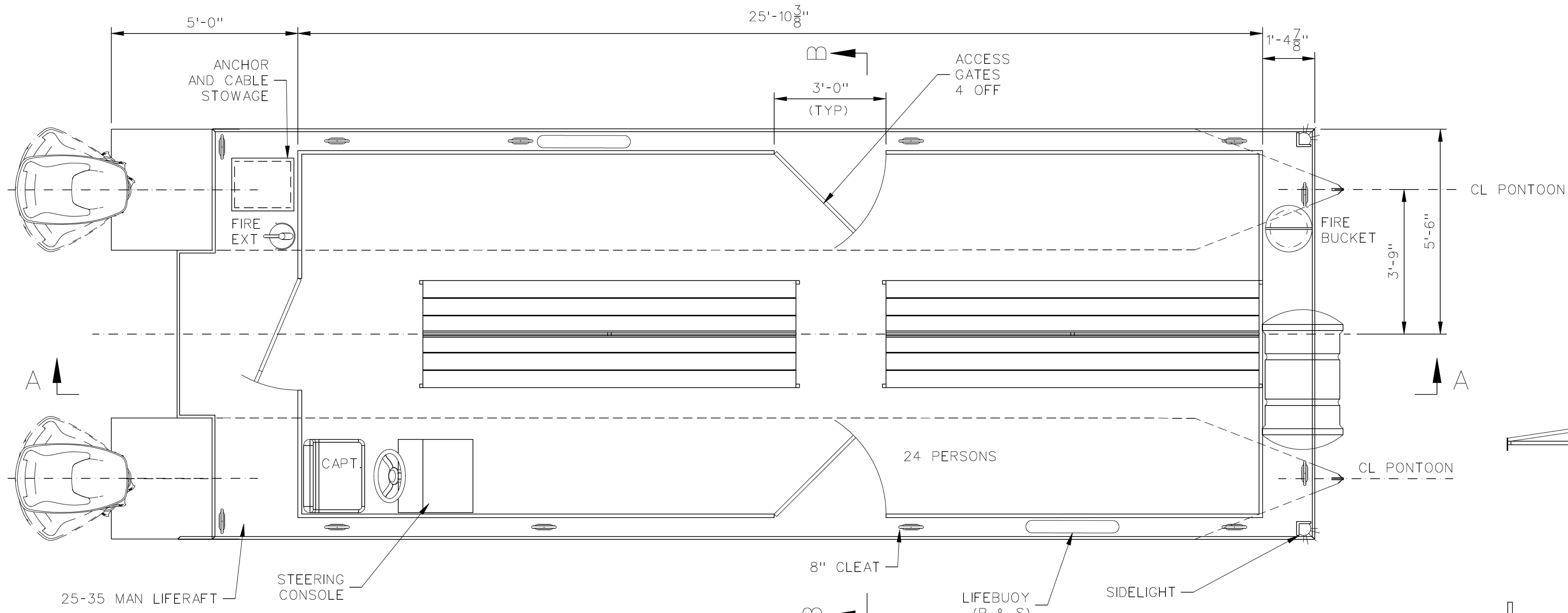
PLAN AT MAIN DECK
